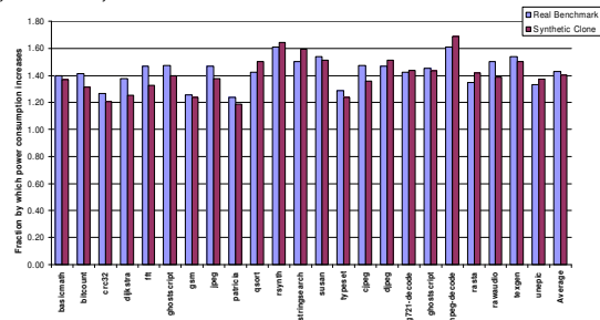
Figure 9. Relative increase in power consumption for real and synthetic benchmarks in response to the design change of doubling the fetch, decode, and issue width.
