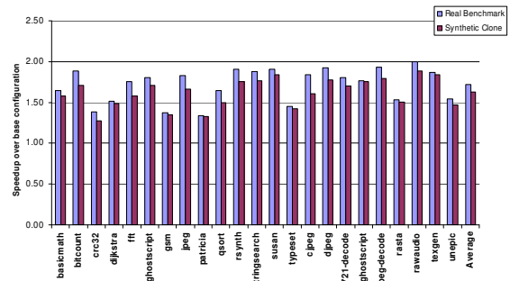
Figure 8. Relative speedup in IPC for real and synthetic benchmarks in response to the design change of doubling the fetch, decode, and issue width.
