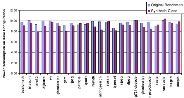
Figure 7. Comparison of the power consumed by the original benchmark and the synthetic benchmark clone on the base configuration.
