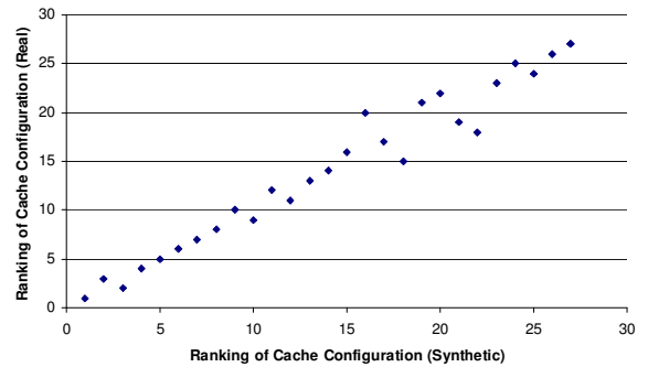
Figure 5. Scatter plot showing ranking of the cache configuration estimated by the synthetic benchmark clone and the real benchmark.
